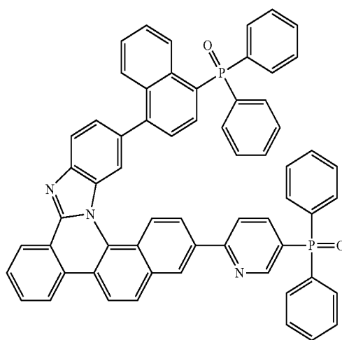
[Compound 3-6]
