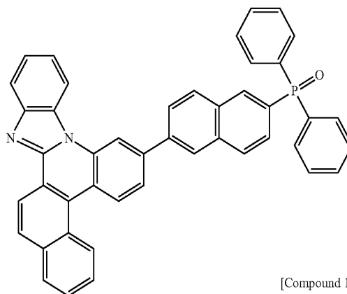
[Compound 1-1]
