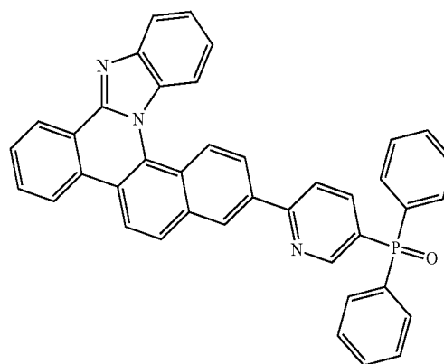
[Compound 1-2]
