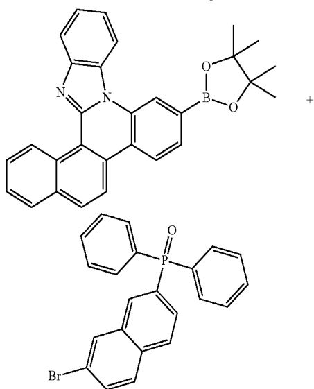
[Structural Formula 1-37E]
