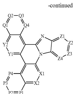
[Chemical Formula 10]
