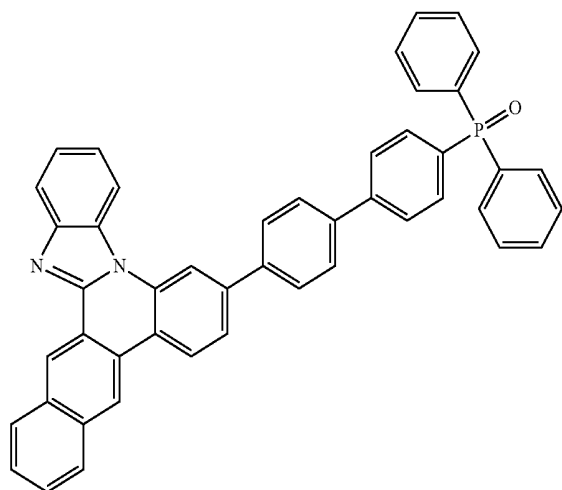
[Compound 1-104]
