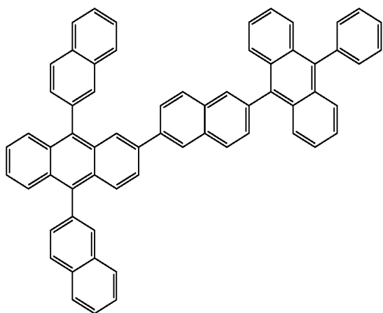
[H2]
