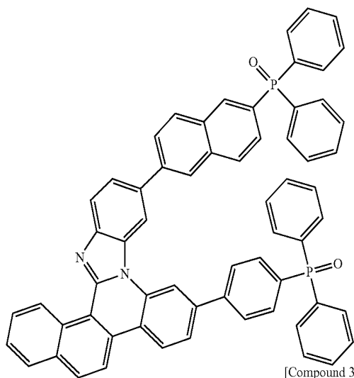
[Compound 3-2]
