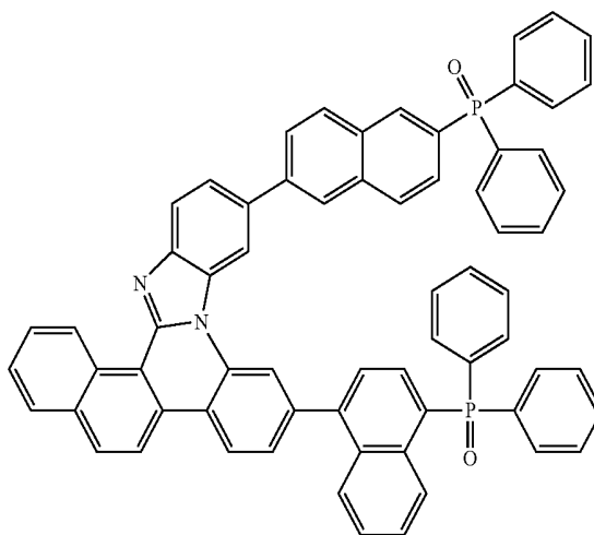
[Compound 3-5]
