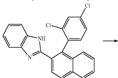
[Structural Formula 1-1B]
