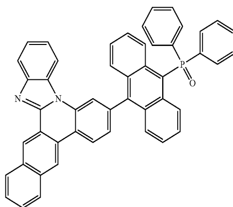
[Compound 1-106]
