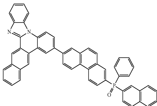
[Compound 1-107]
