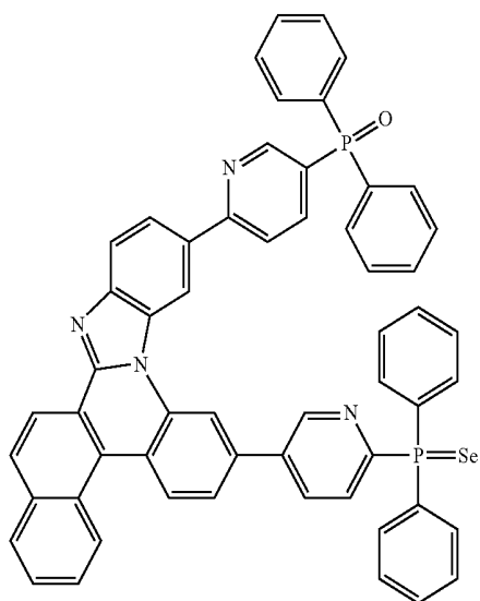
[Compound 3-33]
