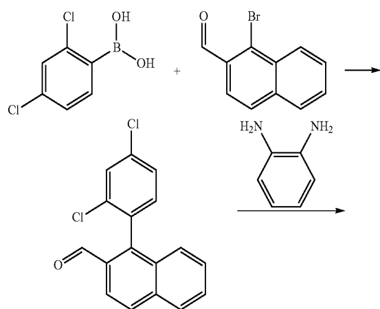
[Structural Formula 1-1A]
