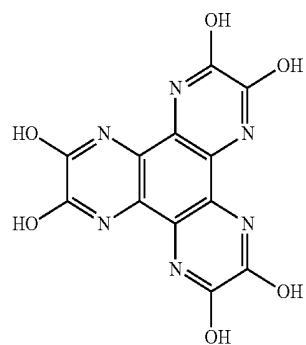
[Hexanitro hexaazatriphenylene]
