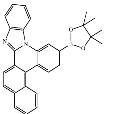
[Structural Formula 1-1D]
