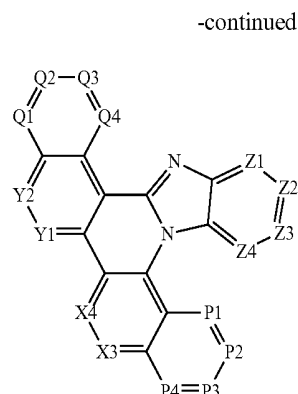
[Chemical Formula 9]
