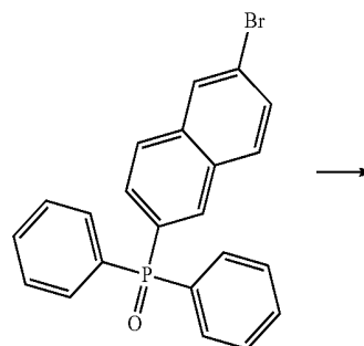
[Structural Formula 1-1D]
