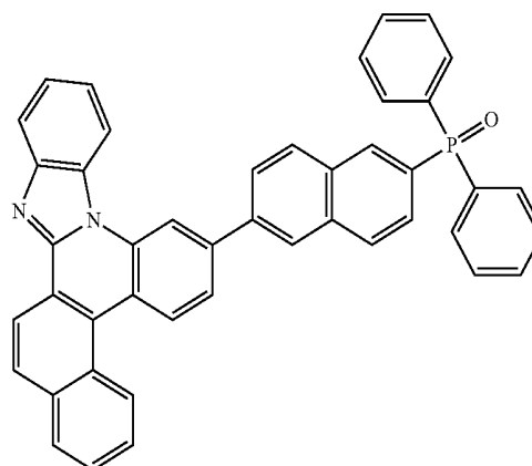
[Compound 1-2]
