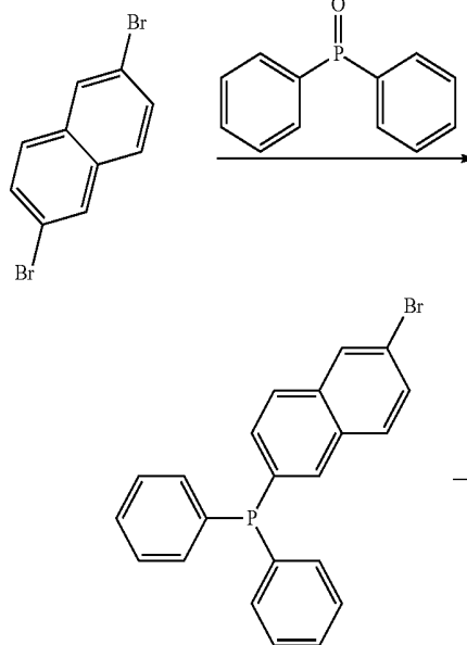
[Structural Formula 1-1E]
