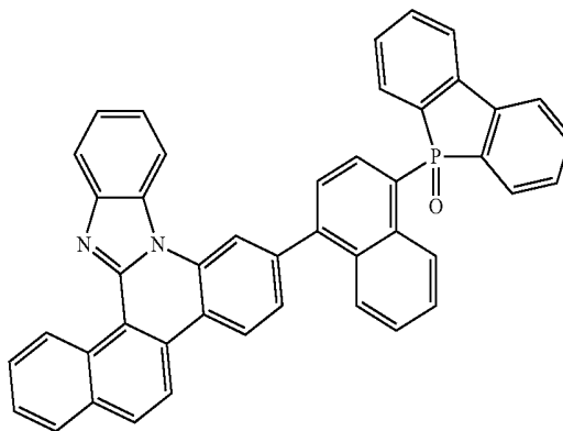
[Compound 4-1]
