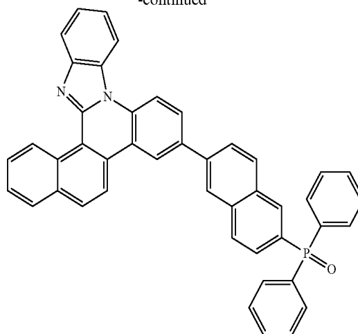
[Structural Formula 1-1F]
