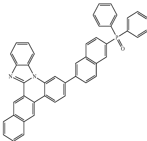
[Compound 1-105]
