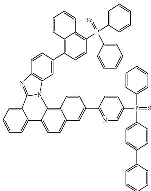
[Compound 3-32]
