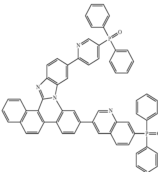
[Compound 3-6]
