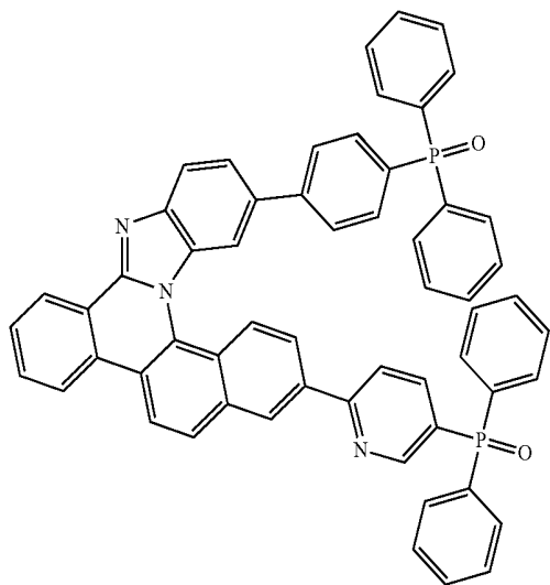
[Compound 3-3]
