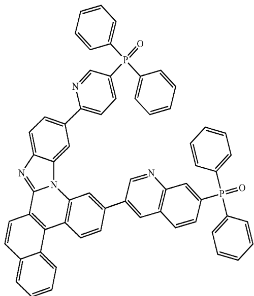
[Compound 3-3]
