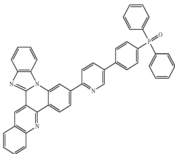
[Compound 1-102]
