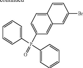
[Structural Formula 1-37E]
