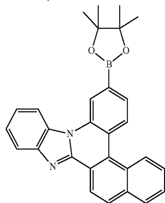
[Structural Formula 1-1D]
