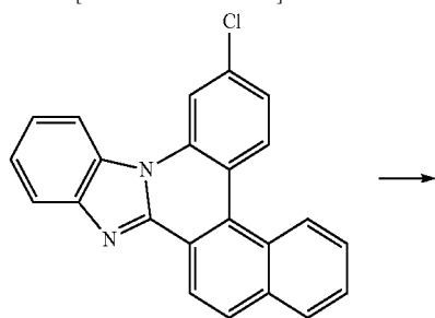
[Structural Formula 1-1C]
