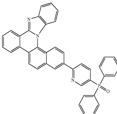
[Compound 1-3]
