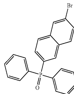
[Structural Formula 1-1F]
