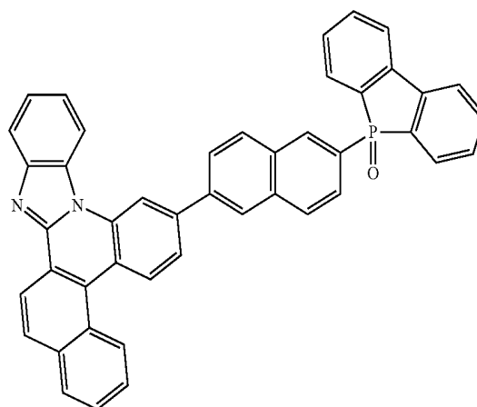
[Compound 4-2]
