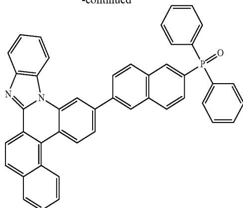
[Structural Formula 1-1F]
