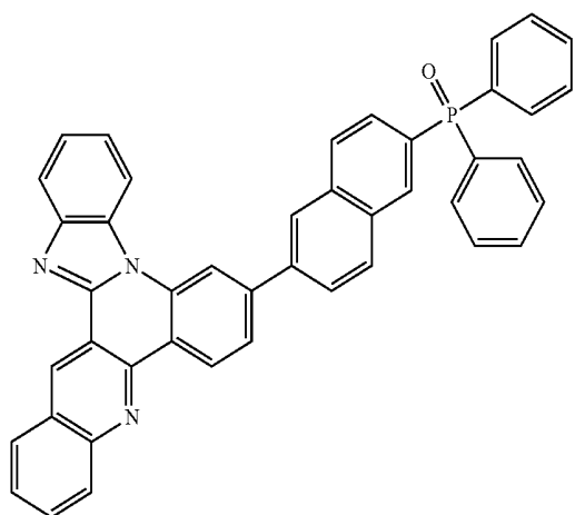
[Compound 1-103]
