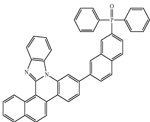
[Structural Formula 1-37F]
